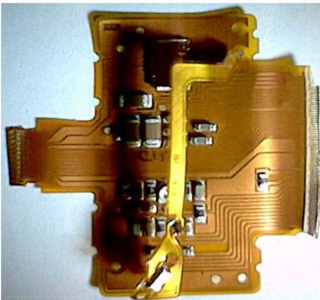
Figure 14B - LG Phone Display Flex (Gilleo teardown)
